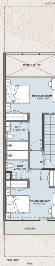
1ST FLOOR
